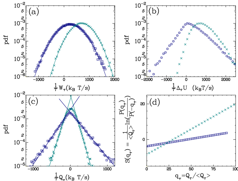
Fig. 2 – TFT. All plots are given for two values of \tau/\tau_\alpha : 0.3 ( \square ) and 1.04 ( \times ). a) PDFs of \frac{1}{\tau} W_\tau . Continuous lines are Gaussian fits. b) PDFs of \frac{1}{\tau} \Delta_\tau U . c) PDFs of \frac{1}{\tau} Q_\tau . Continuous lines are exponential fits for large Q_\tau . d) Functions S(q_\tau) for large heat fluctuations q_\tau computed using exponential fits.
