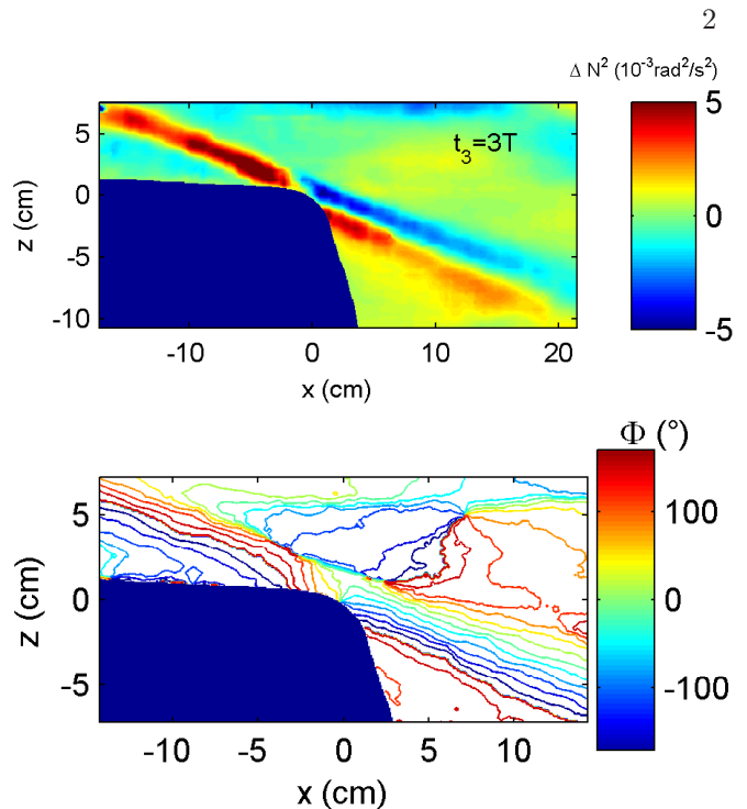
FIG. 2: (Color online) Panel a presents the two-dimensional vertical density gradient, while panel b shows the phase. Both plots have been averaged over one tidal period of the experiment around t = 3T . Horizontal and vertical distances are in cm. The generation point C appears to be an amphidromic point around which the phase of the wave rotates.
