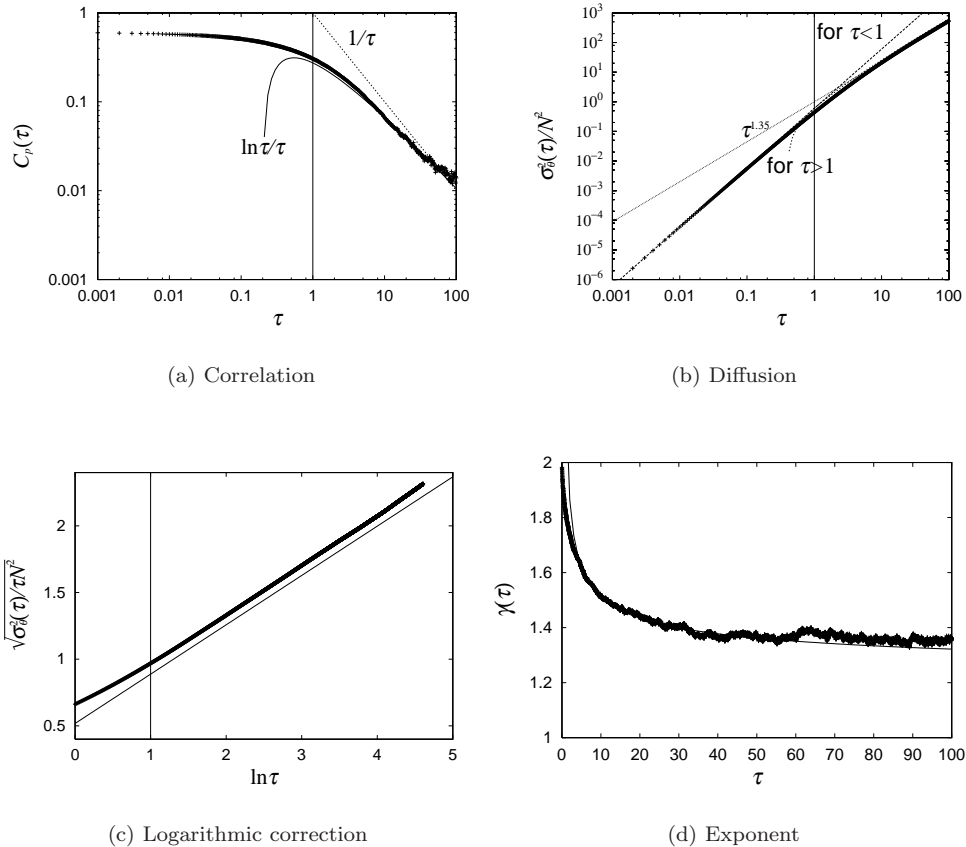
FIG. 4: Check of the theoretical prediction for gaussian stable initial distributions in the case U = 0.8 with N = 10^4 . Points are numerically obtained by averaging 20 realizations. In panel (a), the symbols show the correlation function of momenta. The theoretical prediction, \ln \tau/\tau , is a better approximation than the simpler law 1/\tau . Panel (b) presents the diffusion of angles. Although the diffusion is normal, the straight line \tau^{1.35} wrongly suggests that it is not. See text for explanations and details. Panel (c) shows the quantity \sqrt{\sigma_\theta^2(\tau)/(\tau N^2)} as a function of \ln \tau to confirm the logarithmic correction of the diffusion. The straight line is a guide for the eyes. Finally, panel (d) presents the temporal evolution of the instantaneous exponent \gamma . The dashed line corresponds to relation (12).
