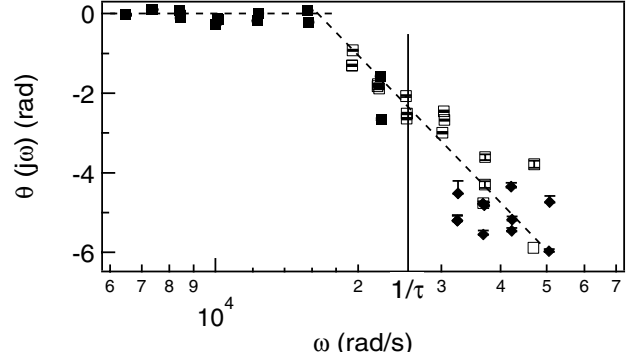
Fig. 10. Phase \theta(j\omega) \equiv \arg[\hat{f}(j\omega_n)] as a function of \omega . The experimental data set is the same as in Figure 9. In order to get a constant phase \theta for \omega < \frac{1}{\tau} , we take t_0 = 2.3 \times 10^{-4} s ( \delta P = 18 Pa, \Phi = 8 mm).
