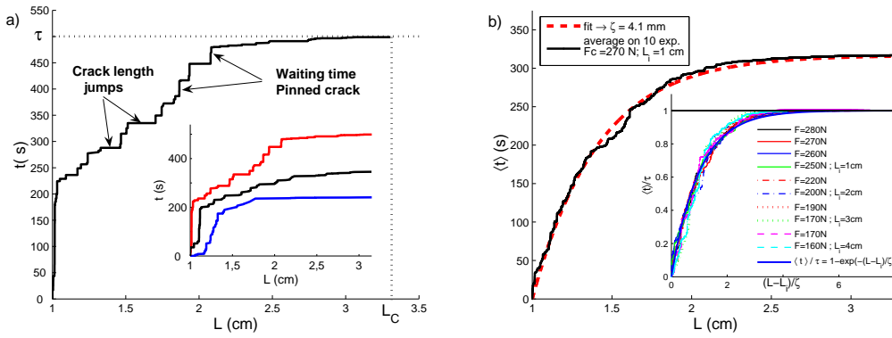
Fig. 3 – a) Typical stepwise growth curve for a creep experiment with an initial crack length L_i = 1\text{ cm} submitted to a constant load F = 270\text{ N} . The lifetime of the sample is \tau = 500\text{ s} and the critical length L_c = 3.3\text{ cm} . In insert, a strong dispersion is observed in crack growth profile and in lifetime for 3 creep experiments realized in the same conditions. b) Statistical average of growth curves for 10 creep experiments realized in the same conditions ( L_i = 1\text{ cm} , F = 270\text{ N} ). The dashed line corresponds to a fit using equation eq. (1) with a single free parameter \zeta = 0.41\text{ cm} . Insert: rescaled average time \langle t \rangle / \tau as function of rescaled crack length (L - L_i) / \zeta for various initial crack lengths and applied stresses. The solid line corresponds to eq. (1).
