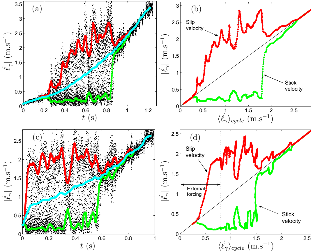
FIG. 15 – (a) and (c), instantaneous peeling velocity |\dot{\ell}_{\gamma}| (black dots), average peeling velocity \langle \dot{\ell}_{\gamma} \rangle_{cycle} (middle curve), average stick (bottom curve) and slip (top curve) velocities as a function of time. (b) and (d) corresponding (respectively to (a) and (c)) average stick and slip velocities as a function of the average peeling velocity. (a) and (b) curves correspond to a spontaneous stick-slip peeling experiment performed with m = 245\text{g} . (c) and (d) curves correspond to a triggered stick-slip peeling experiment performed with m = 195\text{g} .
