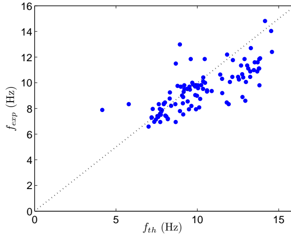
FIG. 8 – Experimental oscillation frequency as a function of the theoretical prediction (cf. equation 2), taking into account the accelerated motion of the load. The data corresponds to different applied masses m = 170, 195, 245, 265\text{g} , various radius 5.60\text{cm} > R > 3.60\text{cm} and different moments during the fall of the mass.
