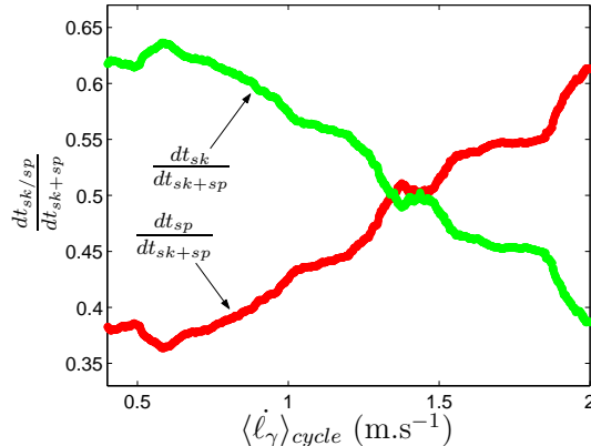
FIG. 17 – Ratio of the stick (light grey/green points) and slip (strong grey/red points) phases duration with the stick-slip duration as a function of the average peeling point velocity for a stick-slip peeling experiment performed with m = 245\text{g} .
