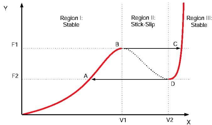
FIG. 1 – Schematic relation between the peeling force f and the peeling velocity v at the peeling crack line. These variables refer to the local dynamics of the peeling point and correspond to the tensile force F and velocity V at the free end of the tape only when the peeling is regular and the peeling angle 90^\circ . The sigmoidal shape is responsible for the hysteretic behavior and therefore for the stick-slip dynamics.
