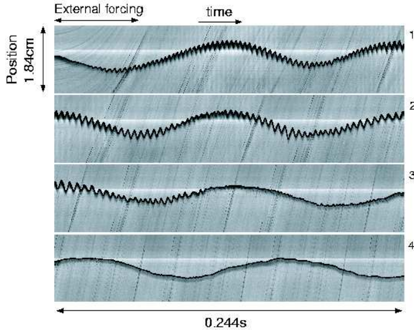
FIG. 9 – Spatiotemporal image of the peeling point region for a triggered stick-slip peeling experiment performed with m = 195\text{g} . The extracted peeling point position has been added in black.
