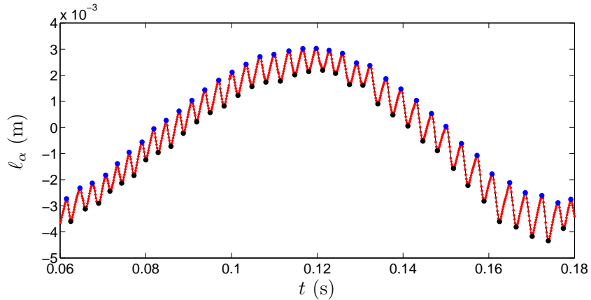
FIG. 10 – Position of the peeling point in the laboratory reference frame, \ell_\alpha , as a function of time for a triggered stick-slip peeling experiment performed with m = 195\text{g} .
