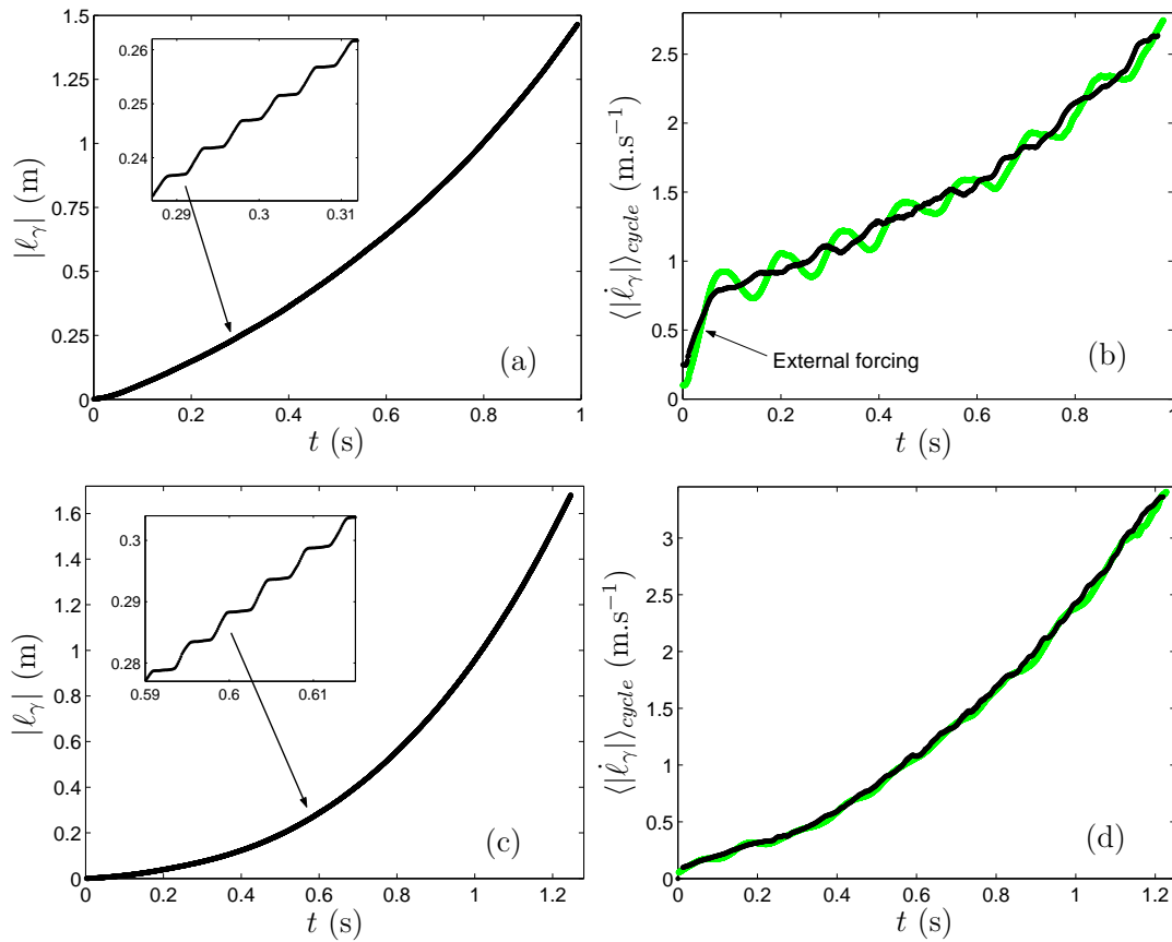
FIG. 13 – (a) and (c), absolute value of the peeling point position in the roller reference frame \ell_\gamma as a function of time. The insets are zooms of these curves in a zone where stick-slip is observed. (b) and (d), corresponding (respectively to (a) and (c)) mean velocity of the peeling point (averaged over a stick-slip cycle) \langle |\dot{\ell}_\gamma| \rangle_{cycle} as a function of time. The light grey (green) curves correspond to the velocity of the roller in the laboratory reference frame \dot{\ell}_\beta . (a) and (b) curves correspond to a triggered stick-slip peeling experiment performed with m = 195\text{g} . (c) and (d) curves correspond to a spontaneous stick-slip peeling experiment performed with m = 245\text{g} .
