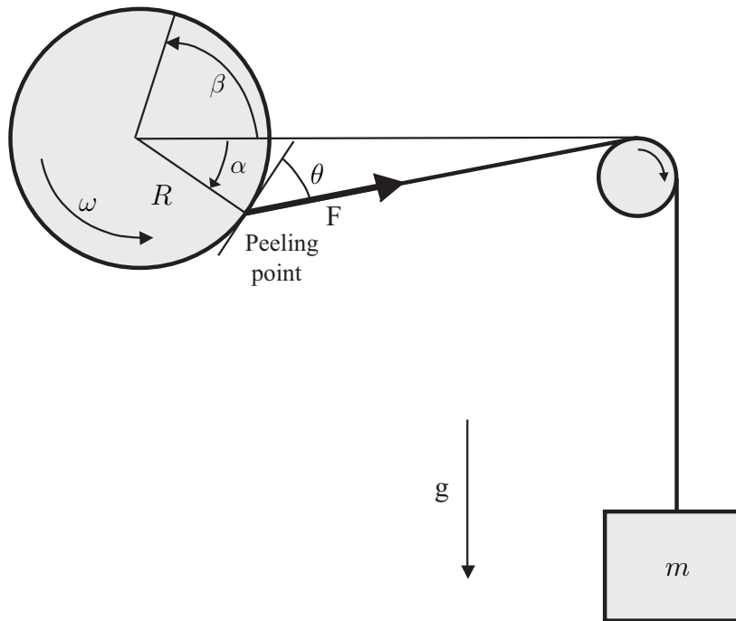
FIG. 3 – Experimental setup and variables. The angles \alpha and \beta are algebraic and oriented trigonometrically. Roller radius : 5.85\text{cm} > 2R > 3.65\text{cm} , roller and tape width : 1.95\text{cm} , tape thickness : 50\mu\text{m} .
