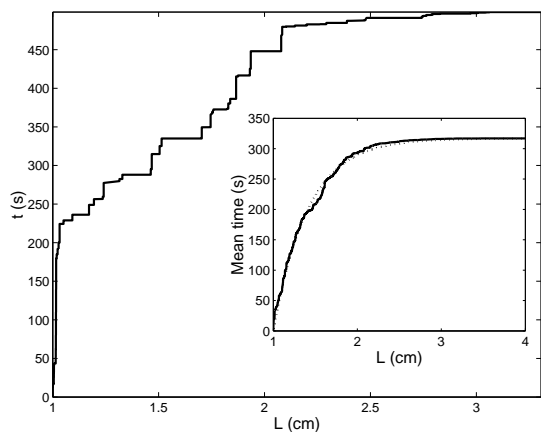
FIG. 1: Time versus crack length for a single experiment showing crack jumps and crack arrest. In insert, average time to reach L (10 experiments with F = 270\text{N} and L_i = 1\text{cm} ). The dotted curve is obtained from integration of eq.(1) [9].
