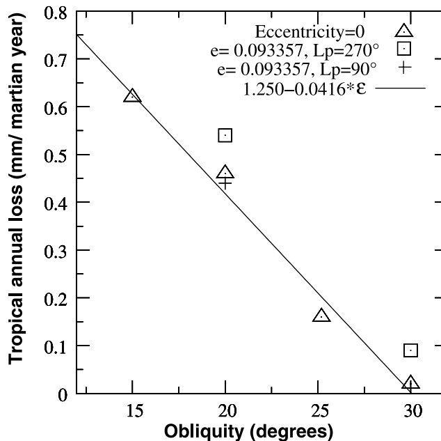
Figure 7. Annual tropical ice loss rates as a function of the obliquity \varepsilon and of orbit’s parameters. The net loss rate of water ice is averaged over the 30°S–30°N latitudinal band. The triangles indicate the loss rates estimated from four LMD GCM simulations with a circular orbit ( e = 0 ). The solid line is its best least squares linear approximation. The squares indicate the net loss rates for L_p = 270^\circ and a present-day eccentricity, while the cross shows the net loss rate of water at L_p = 90^\circ , the present-day eccentricity and a 20° obliquity. For the same orbital configuration, but at 30° obliquity, the tropical reservoir is stable.
