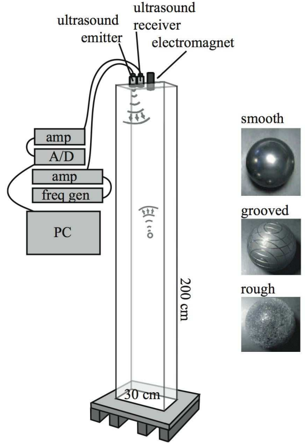
Fig. 1. SETUP: the vertical velocity of falling steel spheres is measured with an ultrasound device. The fluid is tap water, pure or with small amounts of polymeric additives. Smooth, grooved, and rough spheres are tested.
