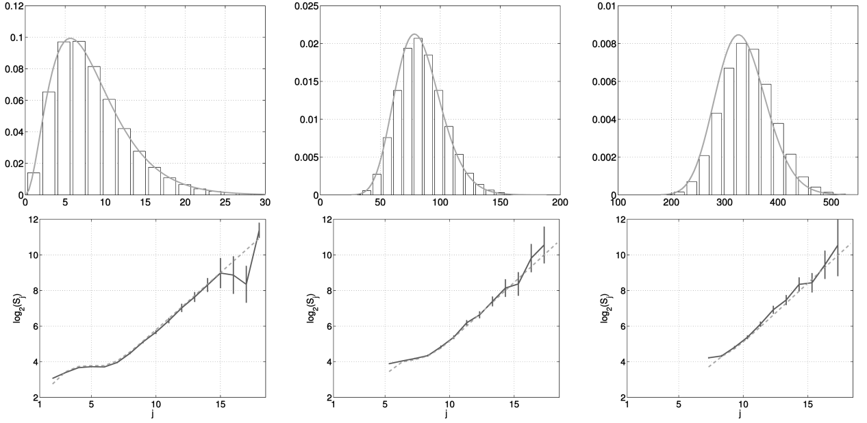
Fig. 7. Synthetic data. \Gamma_{\alpha,\beta} -arfima (\phi, d, \theta) fits for the marginals (top row) and covariances (bottom) of synthetic data for \Delta = 10, 100, 400\text{ms} (left to right). The parameters correspond to those of AUCK-IV .
