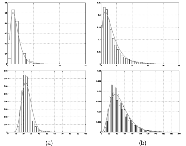
Fig. 9. Marginals. For (a) the DDoS Attack and (b) for the Flash Crowd (right), empirical histograms of X_\Delta and their \Gamma_{\alpha,\beta} fits of the marginals, for \Delta = 2\text{ms} (top) and \Delta = 32\text{ms} (bottom).
