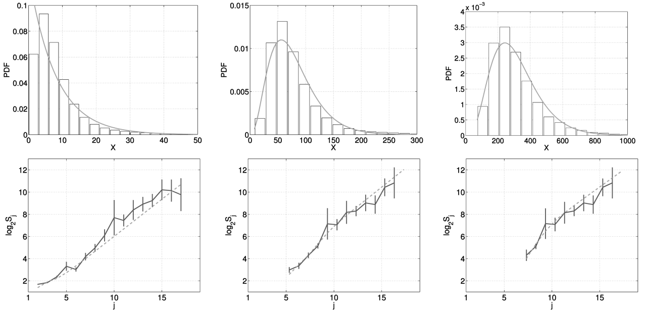
Fig. 5. METROSEC-ref1 . \Gamma_{\alpha,\beta} -arima( \phi, d, \theta ) fits for the marginals (top row) and covariances (bottom) for \Delta = 10, 100, 400 ms (left to right). j = 1 corresponds to 10 ms.
