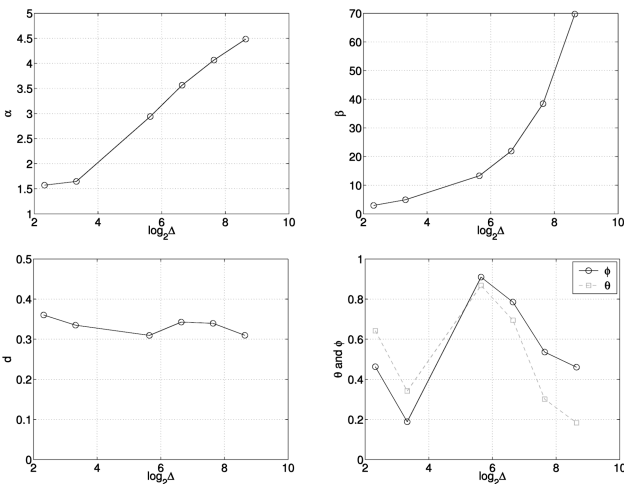
Fig. 6. METROSEC-ref1 . Estimated parameters of \Gamma_{\alpha,\beta} -arima( \phi, d, \theta ), as a function of \log_2 \Delta ( \Delta in ms).
