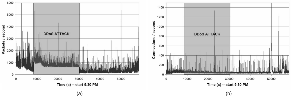
Fig. 1. DDoS Attack. Time series corresponding to the numbers per second of (a) packets and (b) connections.
