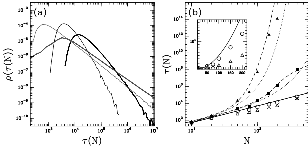
FIG. 4: MFPT \tau(N) (measured in number of steps) for A = l = 200 , \alpha = 2\pi , L = 15000 and \sigma_o = 0.01 . (a) Pdf of \tau(N) calculated for 100000 uncorrelated ( H = 0.5 , black) and LRC ( H = 0.8 , grey) chains for N = 100 (thin) and 200 (thick). (b) Most probable MFPT vs N for H = 0.5 ( \circ ) and 0.8 ( \Delta ); mean MFPT vs N for H = 0.6 ( \blacksquare ) and 0.8 ( \blacktriangle ); the dashed curves correspond to the analytical quenched average (Eq. (10)); the dotted curves correspond to the small displacement approximation (Eq. (11)); the continuous line correspond to the “pure” diffusion case \tau(N) = N^2 .
