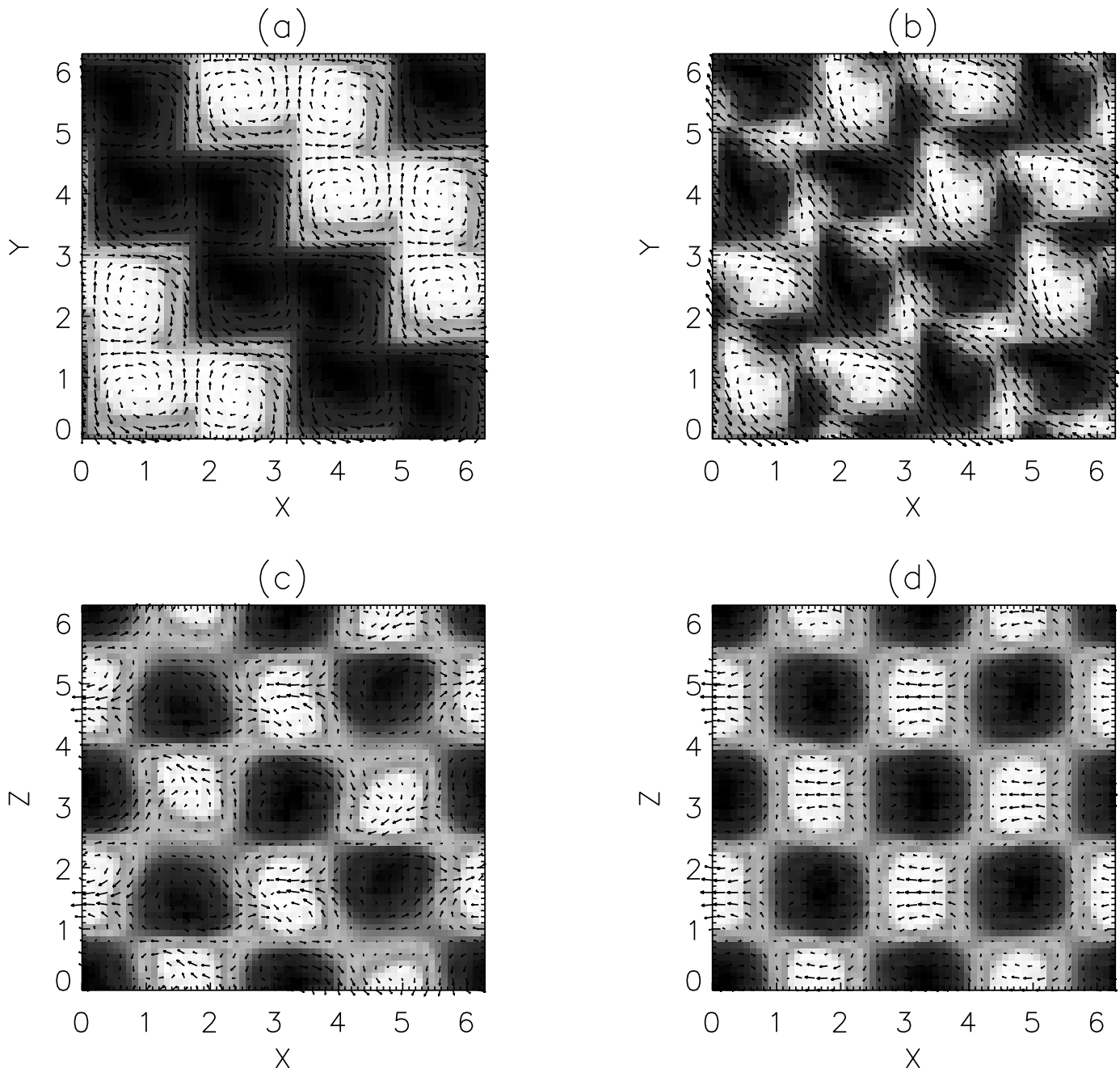
FIG. 5.—Upper panels: Cross-sectional plots of the velocity field in the plane z=0 at (a) t=352 and (b) t=368 , for run A. The arrows show the directions of v_x , v_y , and the colors indicate the values of v_z , positive (light) or negative (dark). Lower panels: Cross-sectional plots of the velocity field in the plane y=\pi/4 at (c) t=352 and (d) t=368 ( v_x , v_z is indicated by the arrows, and v_y by the color). [See the electronic edition of the Journal for a color version of this figure.]
