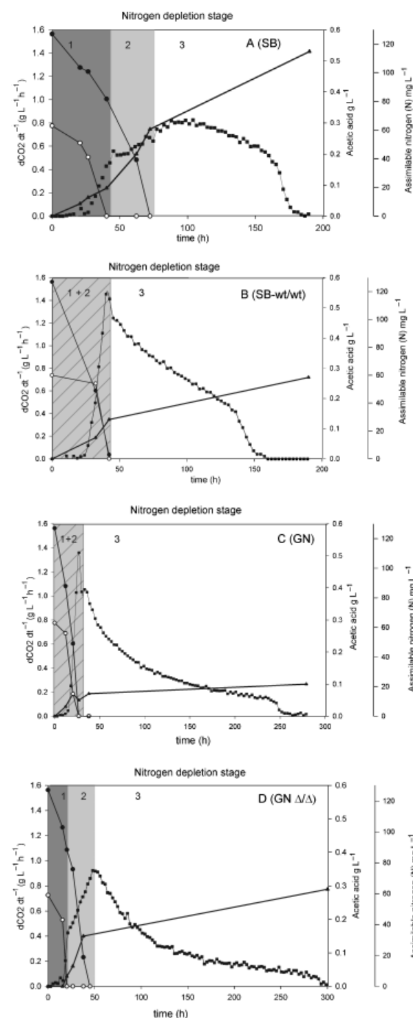
Fig. 7. Relationship between asparagine assimilation, acetic acid production, and CO _2 flux in parent backgrounds. CO _2 production rate (g L ^{-1} h ^{-1} ) was measured for SB ( asp1 -H142/ asp1 -H142), SB-wt ( ASP1 -wt/ ASP1 -wt), GN ( ASP1 -wt/ ASP1 -wt), and GN- \Delta/\Delta ( asp1 - \Delta / asp1 - \Delta ) (plots a, b, c, and d, respectively). The fermentation medium was ASN medium containing asparagine and ammonium. Ammonium ( \circ ), asparagine ( \bullet ) and acetic acid ( \blacktriangle ) were monitored during fermentation. Three nitrogen depletion stages were defined. Stage 1 (dark gray): the medium contained ammonium and asparagine. Stage 2 (light gray): ammonium was depleted and only asparagine remained. Stage 3 (white): the medium contained no more nitrogen sources. For ASP1 strains (b, c), nitrogen depletion stages 1 and 2 were simultaneous (hatched gray). For asp1 mutants, stage 2 occurred after stage 1 and showed overproduction of acetate.
