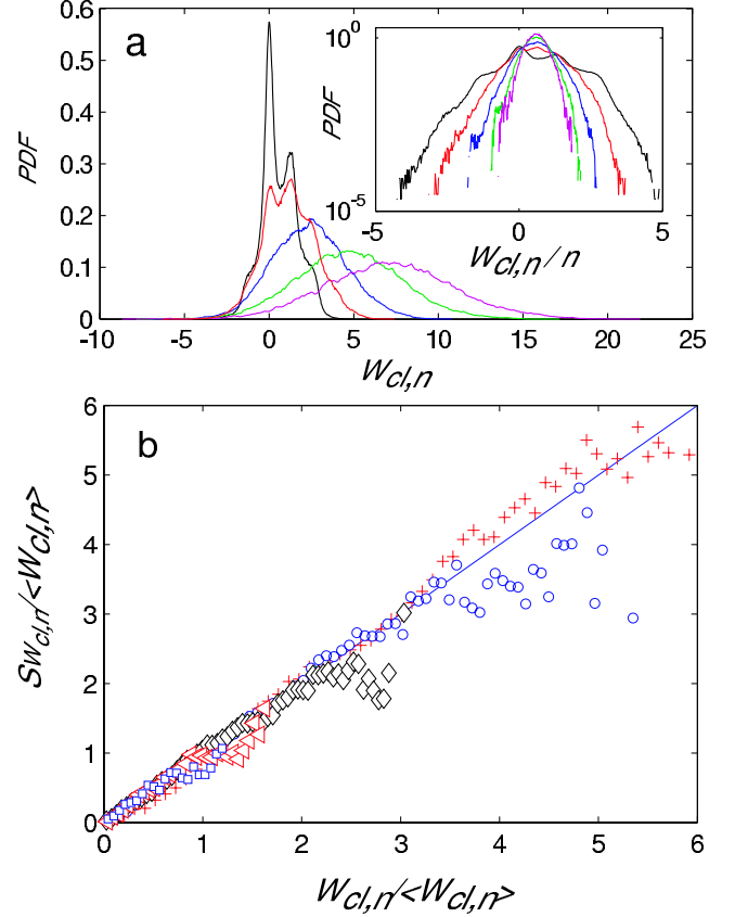
Fig. 8: a) Distribution of classical work W_{cl} for different numbers of period n = 1, 2, 4, 8 and 12 ( f = 0.25 Hz). Inset: Same data in lin-log. b) Symmetry function as function of the normalized work (same symbols as in Fig. 6.)
