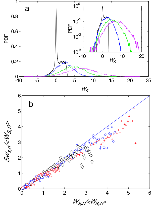
Fig. 6: a) Distribution of stochastic work for different number of period n = 1, 4, 8 and 12 ( f = 0.25 Hz). Inset: Same data in lin-log. b) Normalized symmetry function as function of the normalized work for n = 1 (+), 2 (○), 4 (◇), 8 (△), 12 (□).
