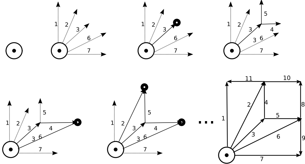
Figure 4: An example derivation of a square by our ESS. Non-terminal collisions are represented by a circle, and non-terminal signals have dangling ends.
