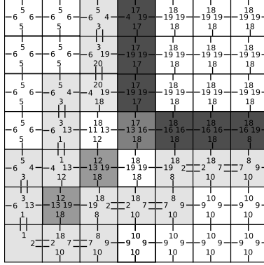
Figure 1: A self-assembling system \mathcal{E} for assembling a square, presented through a 7 \times 7 production
