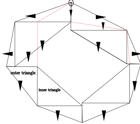
Figure 9: A (tentative) ESS for building polygons with signals
