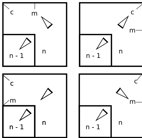
Figure 22: The position of active corner (c) and active middle (m) depending on the orientations of the two last frames
