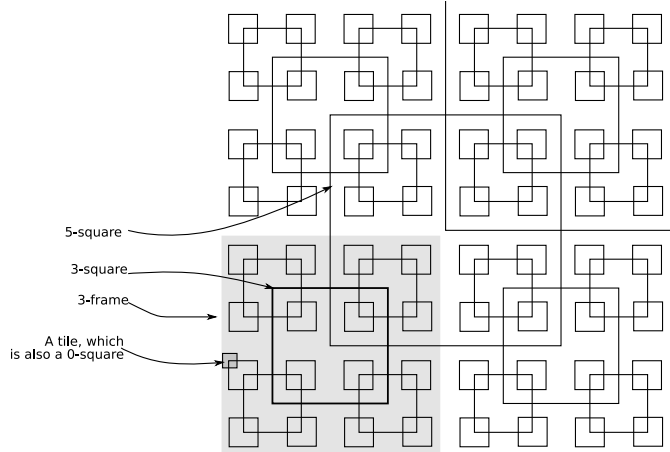
Figure 19: A bird's eye view of a Robinson tiling. The grey frame has direction SW
