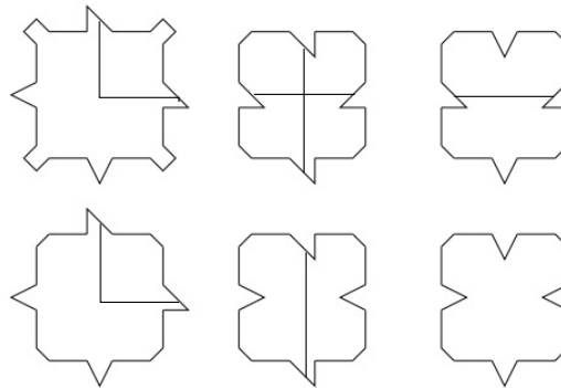
Figure 18: Robinson's tile-set
