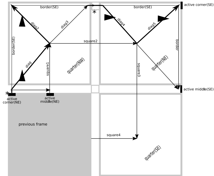
Figure 21: Recursive construction for Robinson frames as an ESS. Signals with a star are one-time signals. This enforces the width 1 of the gap between the four squares. Variants of this figure occur according to the relative directions of the two primary frames which are involved.
