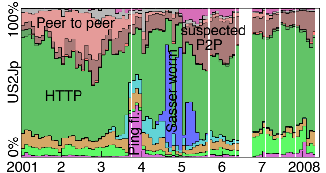
Fig. 2. Applications/anomalies breakdown vs. years. Bottom to top : Ping, DNS, common services, MS vulnerabilities, Sasser, HTTP, broadcast, suspected P2P, identified P2P, other TCP/UDP, GRE.
