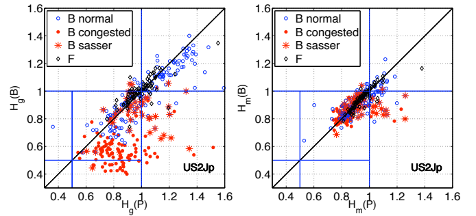
Fig. 6. Scatter plots of H(B) (byte) vs. H(P) (packet). Global (left) and median-sketch (right) estimates (US2Jp). Symbols are: \circ : B without congestion; \bullet : B with congestion; * : B anomaly; \diamond : F .
