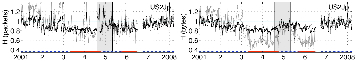
Fig. 5. LRD vs. years. Global (gray lines) and median-sketch (on IPdst) (black lines) estimates of H vs. years 2001-2008.
