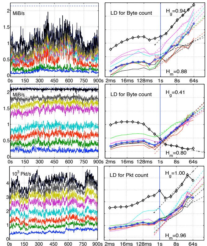
Fig. 4. Robust estimation. Left: Aggregated byte time series (1s) displayed cumulatively by sketch sub-trace; Right: LDs for global traffic (thick line, \diamond ), for sketches (thin lines) and for median-sketch (thick line, \circ ). Top row, B-US2Jp , 2005/07/11, no congestion: Ex1 (Byt). Middle, B-US2Jp , 2003/06/03, with congestion: Ex2 (Byt). Bottom, B-Jp2US , 2004/09/21, with severe anomalies: Ex3 (Pkt).
