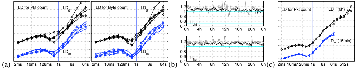
Fig. 7. One day: Statistics (Jp2US). (a) LDs for 15min long traces (Left: Pkt; Right: Byte): Global (black \diamond ) and median-sketch (blue \bullet ). (b) Estimates for H vs. time: Global (gray), median-sketch (black). (c) LDs for 6h-long traces (Jp2US): Average LD over 15-min long traces (blue \bullet ) and LD computed fully on 6h trace (black \diamond ).
