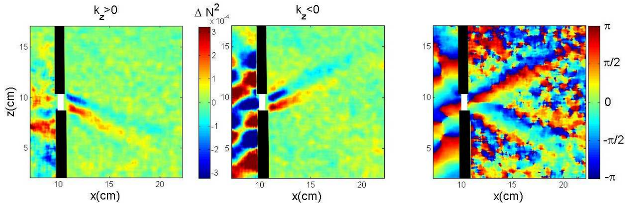
FIG. 12: Small slit case. Hilbert transform of the horizontal density gradient field \rho_x in \Delta N^2 ( \text{rad.s}^{-1} ) 2 filtered at \omega = 0.196 \text{rad.s}^{-1} for a = 2 cm with k_z > 0 (left panel), k_z < 0 (centered panel) and phase of the complete field with all values of k_z (right panel).
