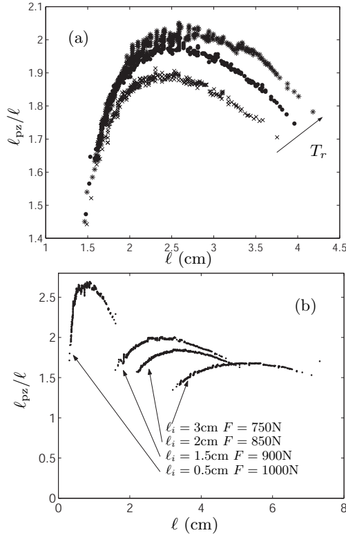
Fig. 13. \ell_{pz}/\ell ratio as a function of the crack length (a) for three experiments performed with the same experimental conditions ( \ell_i = 1.5\text{cm} and F = 900\text{N} ), (b) for four experiments performed with different experimental conditions.
