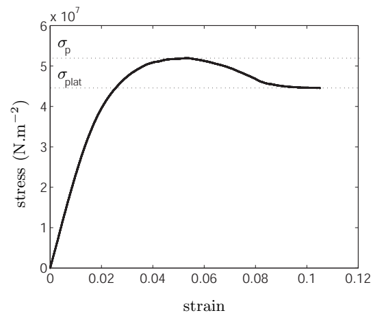
Fig. 1. Stress as a function of strain for a 125 \mu m thick polycarbonate film loaded with a 1.93 \cdot 10^{-4} \text{s}^{-1} strain rate.
