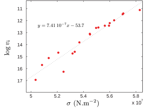
Fig. 8. Natural logarithm of the plastic zone initial velocity as a function of the applied stress. The dotted line is a linear fit.
