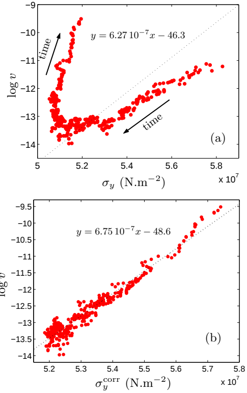
Fig. 15. Natural logarithm of the instantaneous crack growth velocity as a function of (a) the Dugdale-Barenblatt stress and (b) the corrected Dugdale-Barenblatt stress \sigma_y^{\text{corr}} for an experiment performed with F = 900\text{N} and \ell_i = 1.5\text{cm} . In Fig. (a), the dotted line is the result of the Fig. 14 data fit. In Fig. (b), the dotted line is the result of a linear data fit.
