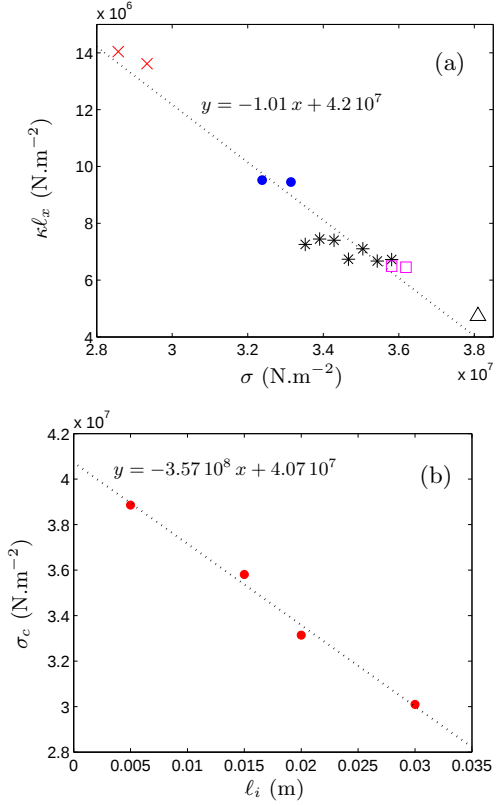
Fig. 17. (a) \kappa\ell_x for various experimental conditions ( \ell_i = 1.5, 2, 3\text{cm} and 2.9 < \sigma < 3.8 \cdot 10^7 \text{N.m}^{-2} ) as a function of the applied stress \sigma . (b) Critical rupture stress \sigma_c as a function of the initial crack length \ell_i . The dotted lines are a linear fit of the data.
