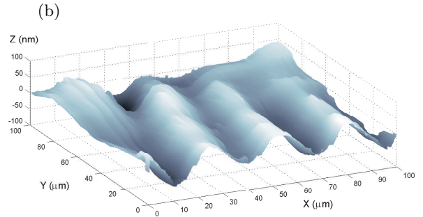
Fig. 9. (a) AFM profile of the plastic zone surface perpendicularly to the striations, (b) AFM three dimensional plot of a plastic zone surface, for a crack tip plastic zone in a 125 \mu\text{m} thick film.
