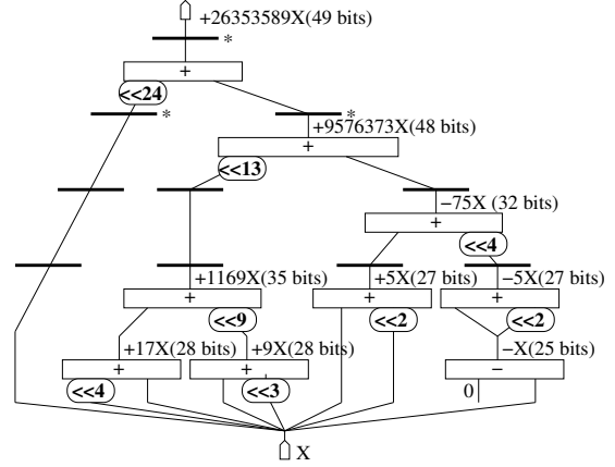
Figure 1: Multiplier by 26353589 pipelined for 200MHz.
