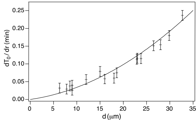
FIG. 9: Derivative dT_0/dr as a function of the sample thickness d . The solid line is the best fit to Eq. 11 by taking \gamma_1 = 0.075 Pa.s.
