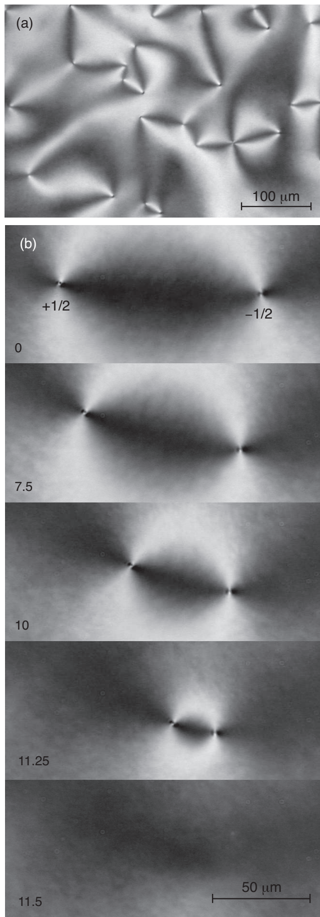
FIG. 1: a) Texture observed at the compensation temperature after a quench from the isotropic liquid. b) Sequence of photographs showing the spontaneous collapse of two \pm 1/2 disclination lines. Note the +1/2 defect moves faster than the -1/2 defect. Time is given in min at the bottom left hand side of the photographs. d = 10 \mu\text{m} . Crossed polarizers.
