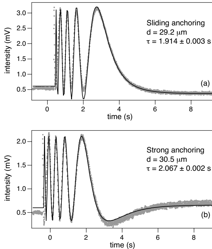
FIG. 3: Optical transmittance measured at T = T_c between crossed polarizers at 45^\circ of the anchoring direction as a function of time after switching off the voltage. Points are experimental and correspond to several curves measured at different places in the sample. The solid line is the best fit to the numerical model. a) Type I sample; b) Type II sample.
