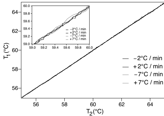
FIG. 5: Temperature of the side wire as a function of the temperature of the middle wire. The curves measured at \pm 2^\circ\text{C}/\text{min} are superimposed (within the experimental noise) whereas those measured at \pm 7^\circ\text{C}/\text{min} are systematically shifted by about 0.1^\circ\text{C} . Note that these curves are noisier than in Fig. 4 because of the use of the scanner card.
