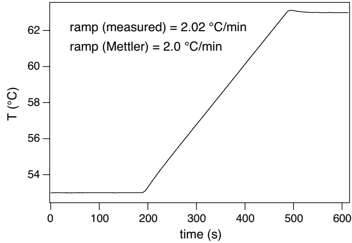
FIG. 4: Temperature profile measured in situ with the tungsten wire. The measured value of the temperature ramp is here slightly larger than its nominal value given by the Mettler oven. This difference increases when the ramp is faster, but never exceeds 5%.
