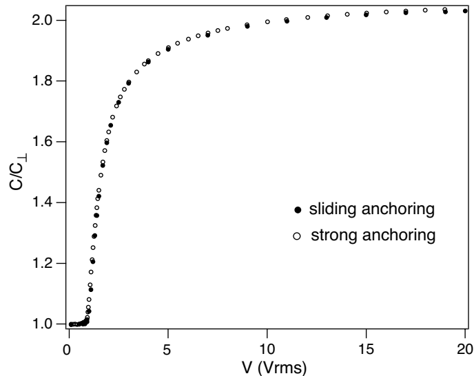
FIG. 2: Capacitance as a function of the applied voltage ( f = 10 kHz) measured at the compensation temperature T_c in a standard planar sample and in a sample treated on one plate for sliding anchoring. The curves superpose within experimental errors.
