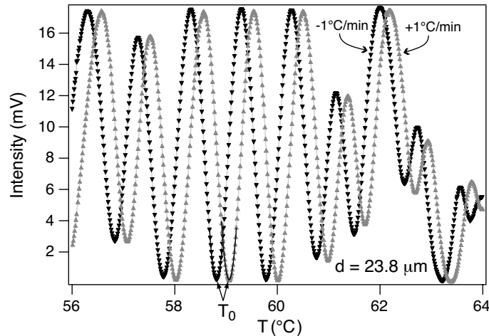
FIG. 7: Curves of optical transmittance measured between crossed polarizers as a function of temperature for two ramps of equal amplitude, but opposite signs. Temperatures T_0 are obtained by fitting with parabolas (solid lines) the local minima.
