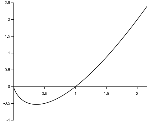
Figure 4: Graph of the function v \mapsto v \log_2(v) .
