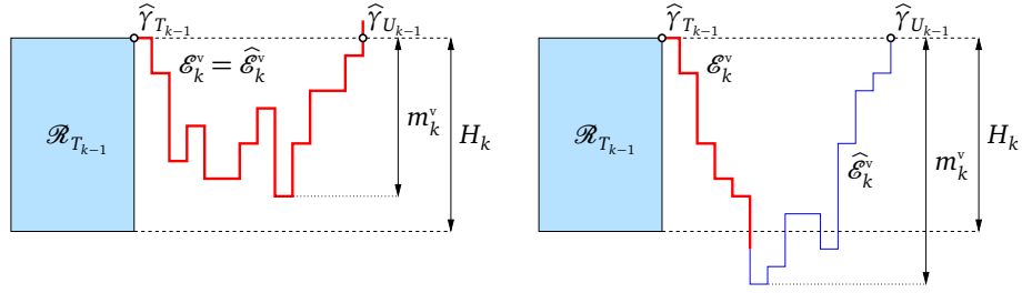
Figure 5: The construction of the vertical excursion \mathcal{E}_k^v of \gamma . from the vertical excursion \hat{\mathcal{E}}_k^v of \hat{\gamma} . When \hat{\mathcal{E}}_k^v is compatible with \mathcal{R}_{T_{k-1}} , it is kept (left); when it is not compatible, it is truncated (right).
