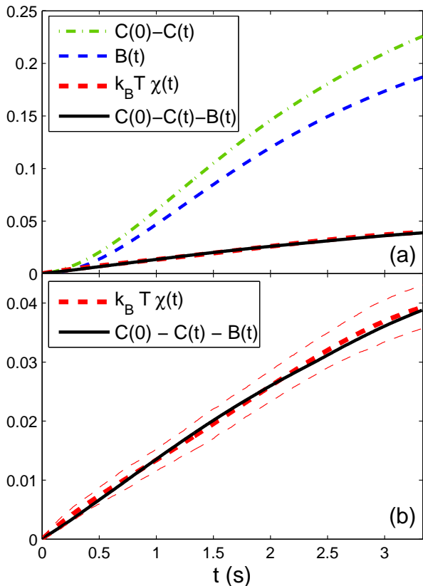
Figure 2: (a) Comparison between the different terms needed to verify Eq. (7), as functions of the time lag t . (b) Expanded view of the comparison between the curves C(0)-C(t)-B(t) and k_B T \chi(t) shown in Fig 2(a). The thin red dashed lines represent the error bars of the measurement of the integrated response.
