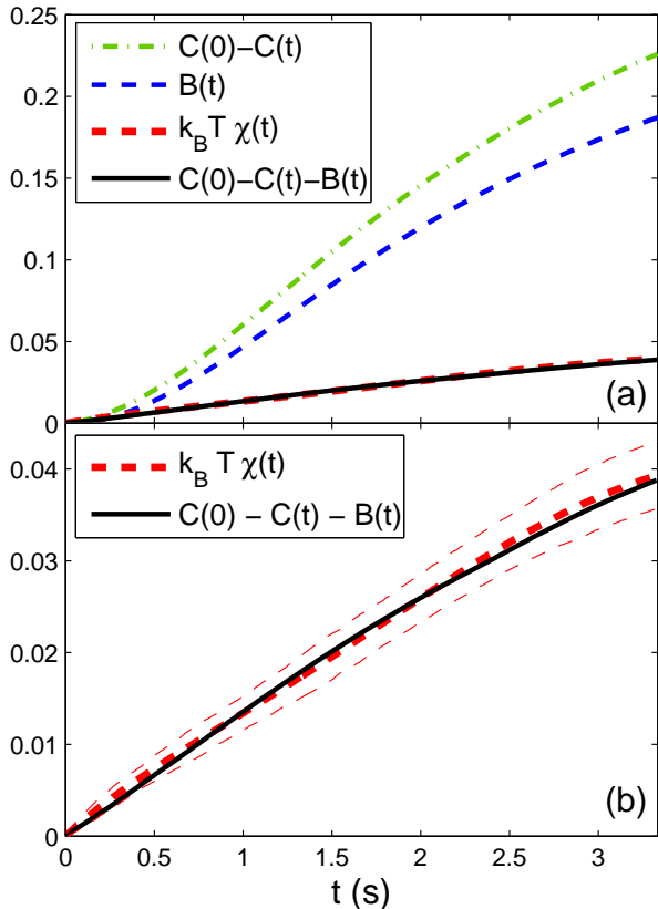
Figure 2: (a) Comparison between the different terms needed to verify Eq. (7), as functions of the time lag t . (b) Expanded view of the comparison between the curves C(0)-C(t)-B(t) and k_B T \chi(t) shown in Fig 2(a). The thin red dashed lines represent the error bars of the measurement of the integrated response.
