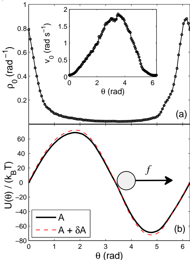
Figure 1: (a) Invariant probability density function of the angular position of the particle in NESS. Inset: Mean local velocity of the particle. (b) Profile of the potential U(\theta) . The arrow indicates the direction of the non-conservative force f .
