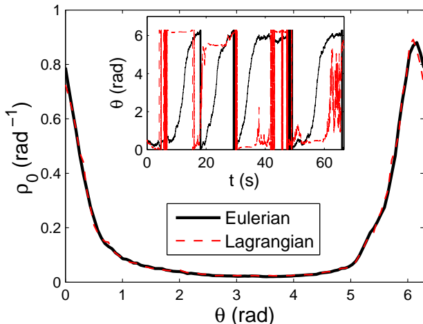
Figure 4: Invariant density of the angular position measured in the Eulerian frame (same as in Fig. 1(b)) and in the Lagrangian frame. Inset: example of a trajectory measured in both frames.
