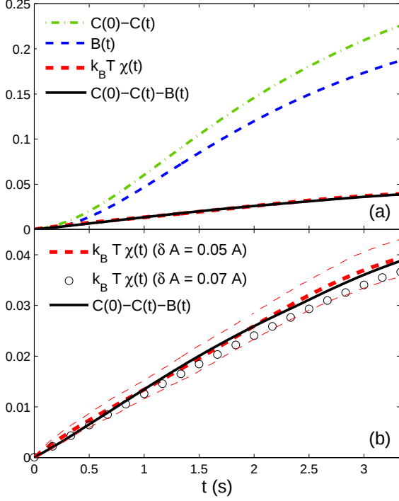
Figure 2: (a) Comparison between the different terms needed to verify Eq. (7), as functions of the time lag t . (b) Expanded view of the comparison between the curves C(0) - C(t) - B(t) and k_B T \chi(t) shown in Fig 2(a). The thin red dashed lines represent the error bars of the measurement of the integrated response.
