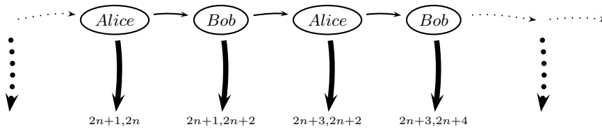
Fig. 4. The strategy “always give up” for the dollar auction game (payoffs are 100v minus the numbers)
