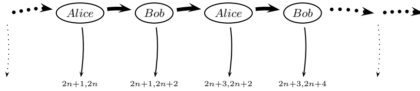
Fig. 3. The strategy “never give up” for the dollar auction game (payoffs are 100v minus the numbers)
