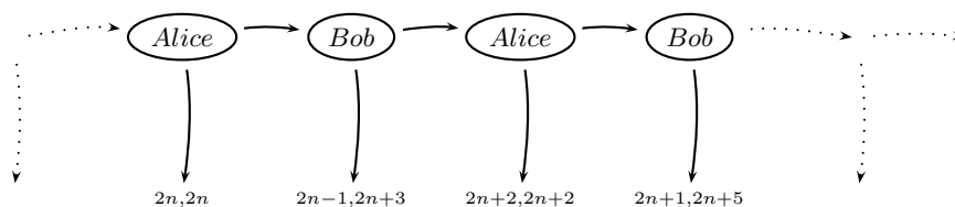
Fig. 5. The centipede game
