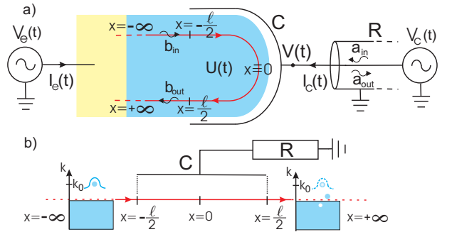
FIG. 1: (Color) (a) Two terminal device built from an edge channel coupled to an RC circuit. In the interaction area |x| \leq l/2 , the edge channel (in red) at internal potential U(t) is capacitively coupled to the gate of capacitance C at potential V(t) . (b) A single electron is injected in the x < -l/2 region and propagates along the edge channel. Interactions within |x| \leq l/2 create electron/hole pairs within the edge channel and photons in the RC circuit leading to decoherence.
