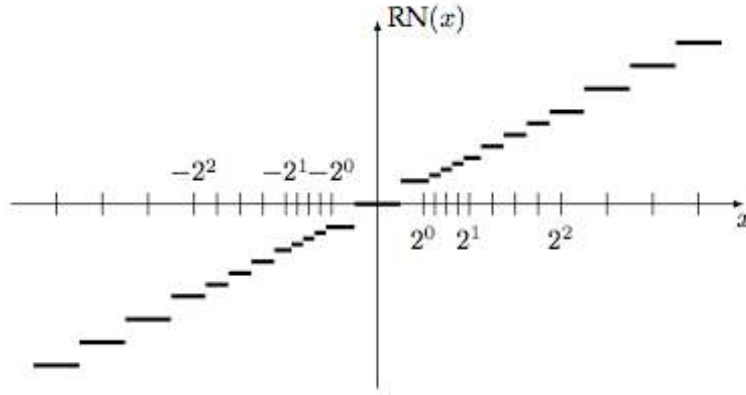
Figure 1: The \text{RN}(x) function for radix \beta = 2 and precision p = 2 .
