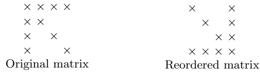
Fig. 1. Ordering affects the sparsity during elimination.
