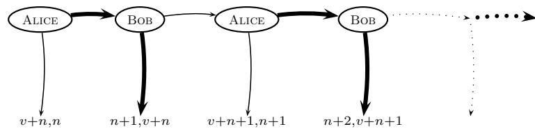
Figure 4: Three strategy profiles
