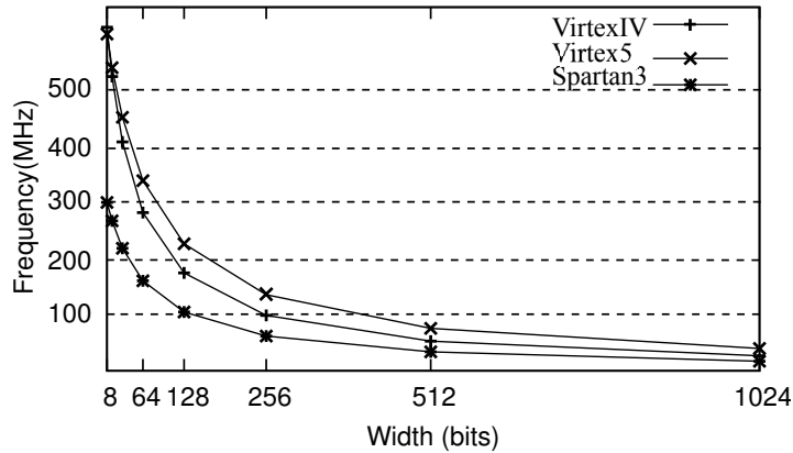
Figure 3: Ripple-Carry Addition Frequency for VirtexIV, Virtex5 and Spartan3E
