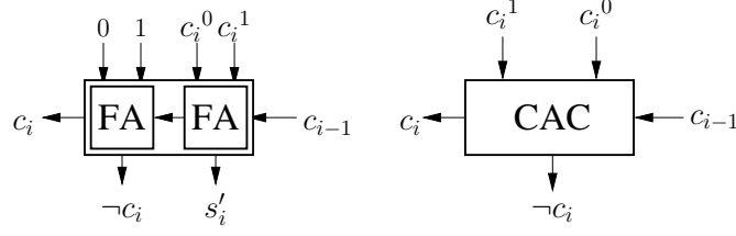
Figure 7: Carry-Add-Cell (CAC) implementation and representation
