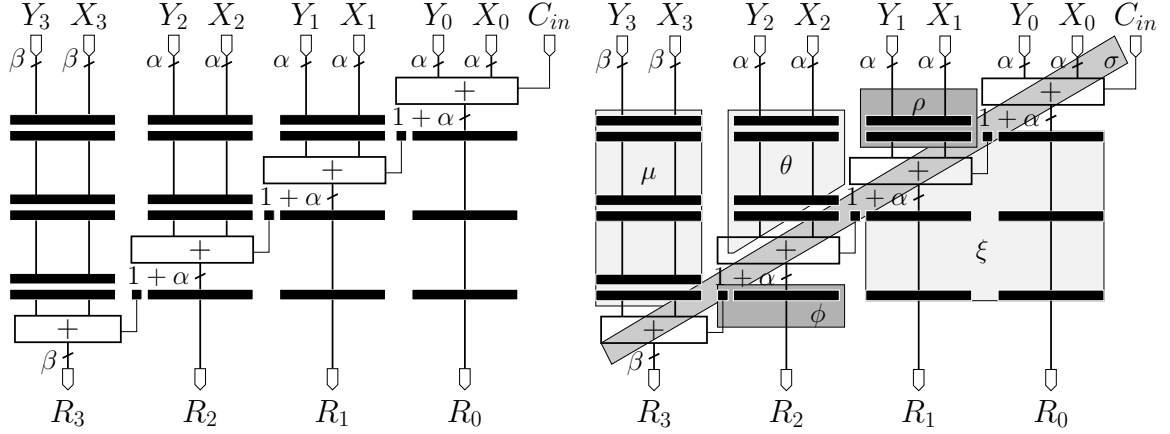
Figure 4: Classical addition architecture [6] Figure 5: Annotated classical architecture
