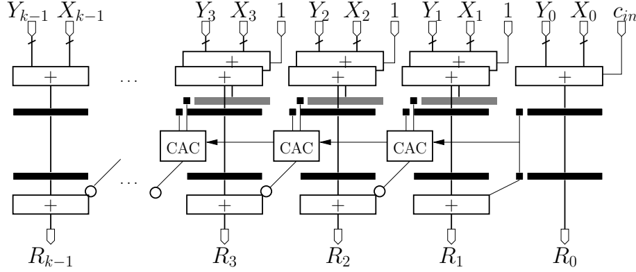
Figure 8: Short-Latency Addition architecture
