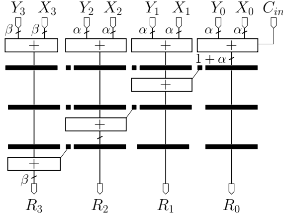
Figure 6: Proposed FPGA architecture
