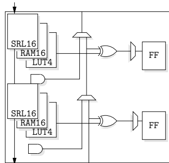
Figure 2: sliceM (VirtexII-Pro, Spartan3 and Virtex-4)
