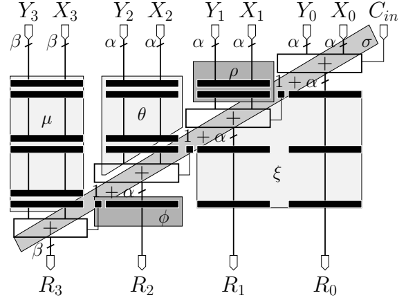
Figure 5: Annotated classical architecture
