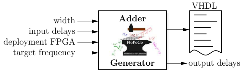
Figure 1: FloPoCo adder generator
