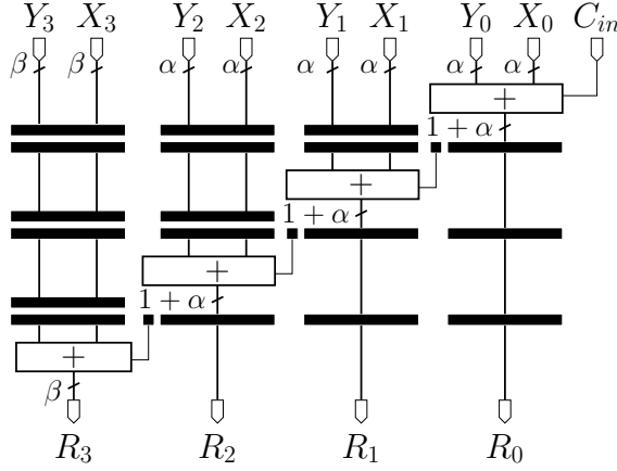
Figure 4: Classical addition architecture [6]
