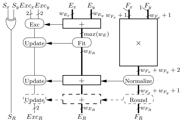
Figure 1: The architecture of a flexible floating-point multiplier
