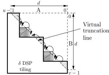
Figure 5: Tiling truncated multiplier using DSPs and soft-core multipliers
