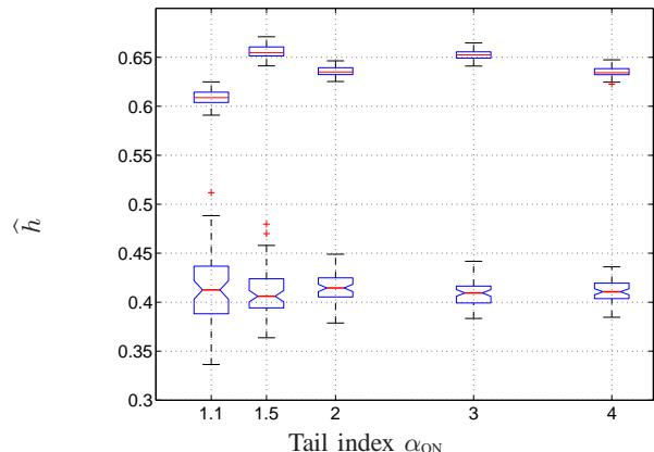
Fig. 10. Fine scale scaling exponent h estimates on aggregated traffic time series ( \Delta = 100 \mu\text{s} ). For different values of the tail index \alpha_{\text{ON}} governing the flow size distributions, h is estimated by linear regression of Log-diagrams (see Fig. 6) over the scale range [0.2 - 5] \text{ ms} . Notched box-plots correspond to UDP protocol, regular box-plots to TCP protocol.
