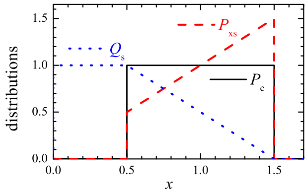
FIG. 20: (Color online): The stationary distribution Q_s(x) (blue dotted line), and the corresponding, numerically obtained, distribution of static thresholds P_{xs}(x) (red broken line) for the rectangular distribution P_c(x) (solid line).
