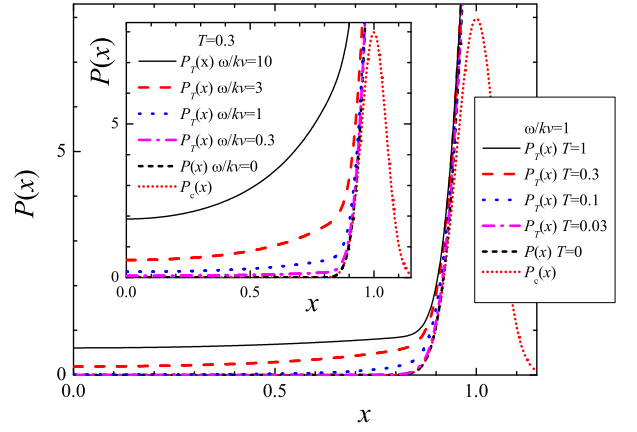
FIG. 8: (Color online): The rate P_T(x) for soft contacts at different temperatures T = 0 (black short dashed), 0.03 (magenta dash-dotted), 0.1 (blue dotted), 0.3 (red dashed) and 1 (black solid curve) for a given velocity, \omega/kv = 1 . Inset: the rate P_T(x) at different velocities \omega/kv = 0 (black short dashed), 0.3 (magenta dash-dotted), 1 (blue dotted), 3 (red dashed) and 10 (black solid curve) for a fixed temperature T = 0.3 . The red short-dotted curve shows the distribution P_c(x) (Gaussian with \bar{x}_s = 1 and \sigma_s = 0.05 ).
