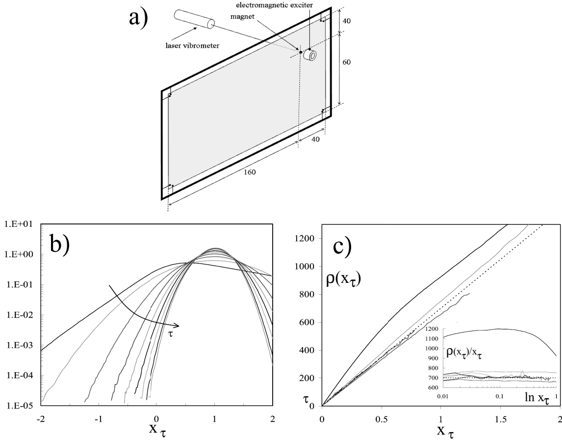
Figure 16: Mechanical waves in a metallic plate (from ref.[57]). a) Schematic diagram of the experiment. A steel plate is suspended to the frame. Dimensions are in cm. The electromagnetic exciter produce et local forcing of the plate vibrations. A laser vibrometer measures the normal velocity at the excitation point. b)and c) Results on the periodic forcing. (b) Pdfs of the injected power on the time durations of \tau for \tau = 3.5ms, 6.5, 13.5, 20, 26.5, 33.5, 40, 47.5, 52ms (c) Functions \rho(x_\tau) = (1/\tau) \log(P(x_\tau)/P(-x_\tau)) obtained from the Pdfs of (b). Inset: compensated value \rho(x_\tau)/x_\tau in a semi log plot. In (c) the dashed line corresponds to a linear law of slope \langle \sigma \rangle = 700Hz .
