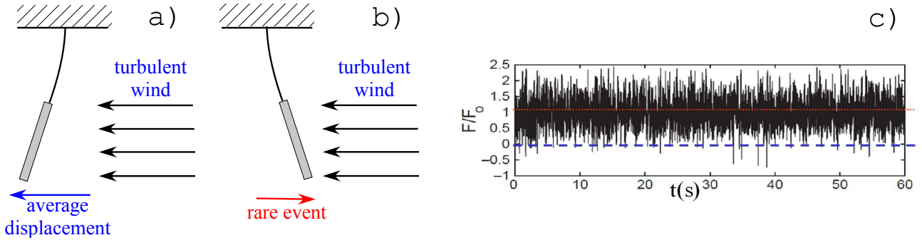
Figure 2: a) and b) Schematic representation of an object suspended by an elastic beam and submitted to the pressure of a turbulent wind a) average behavior b) rare event. c) Time evolution of the measured instantaneous force exerted by the turbulent wind on the object. The details of this experiment can be found [4]
