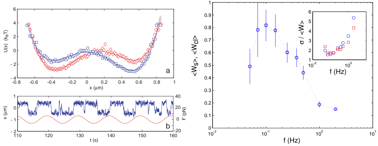
Figure 13: a) The perturbed potential at t = \frac{1}{4f} and t = \frac{3}{4f} . b) Example of trajectory of the glass bead and the corresponding perturbation at f = 0.1 Hz. c) Injected energy in the system over a single period as a function of the driving frequency ( W_s \square and W_{cl} \circ ). The error bars are computed from the standard deviation of the mean over different runs. Inset: Standard deviations of work distributions over a single period normalized by the average work as a function of the frequency (same symbols).
