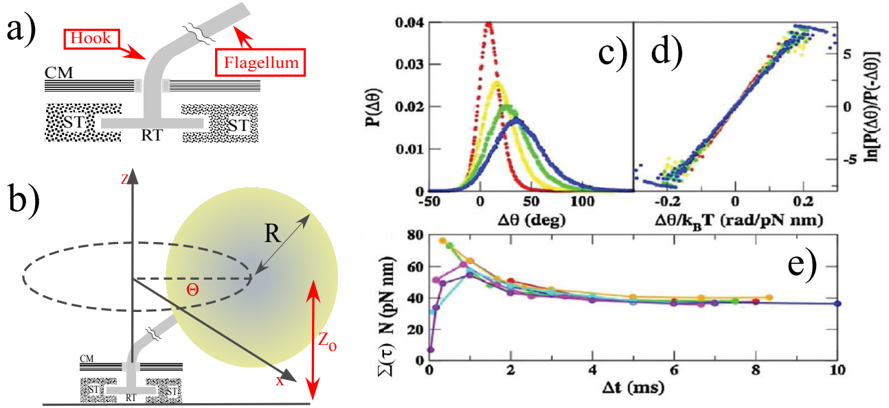
Figure 15: Molecular motor. a) Schematic diagram of a molecular motor composed by a stator and rotor. Sequential chemical reactions between the stator and the rotors produce the motion. (CM) indicate the cellular membrane. b) A bead of about 1 \mu\text{m} is glued to the flagellum in order to follow its rotation with a standard microscope (drawing not to scale). The figures c),d) and e) (taken from ref.[55]) illustrate the results of a measure. c) Pdfs for several \tau of \Delta\theta_\tau . d) Symmetry function extracted from the Pdfs of c). e) Slopes N\Sigma(\tau) of the symmetry function as a function of \tau . The different colors pertain to different experimental conditions. Notice the convergency to an unique value of N for large \tau .
