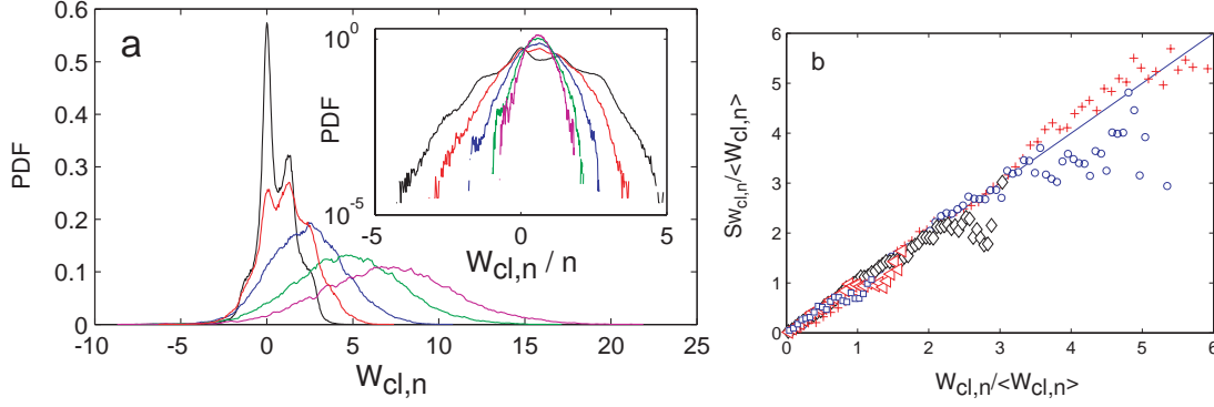
Figure 14: a) Distribution of classical work W_{cl} for different numbers of period n = 1, 2, 4, 8 and 12 ( f = 0.25 Hz). Inset: Same data in lin-log. b) Symmetry function as function of the normalized work (same symbols as in a.)
