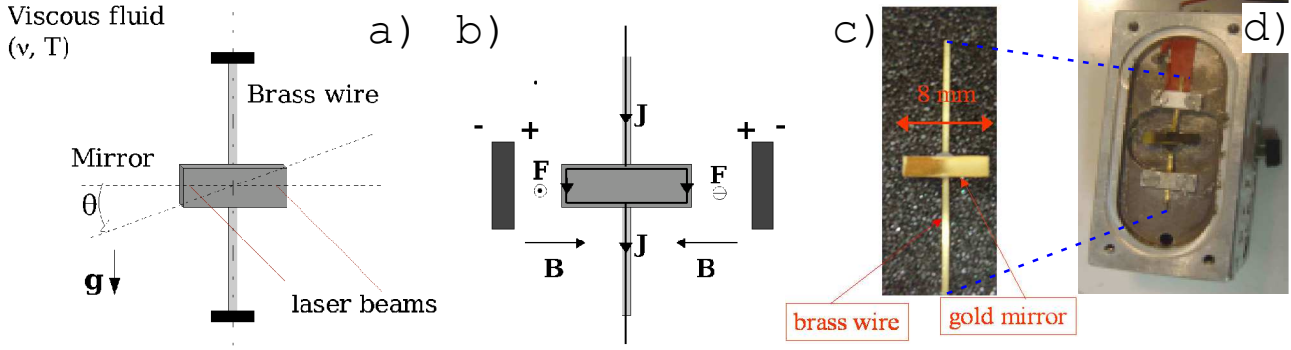
Figure 3: a) The torsion pendulum. b) The magnetostatic forcing. c) Picture of the pendulum. d) Cells where the pendulum is installed.
