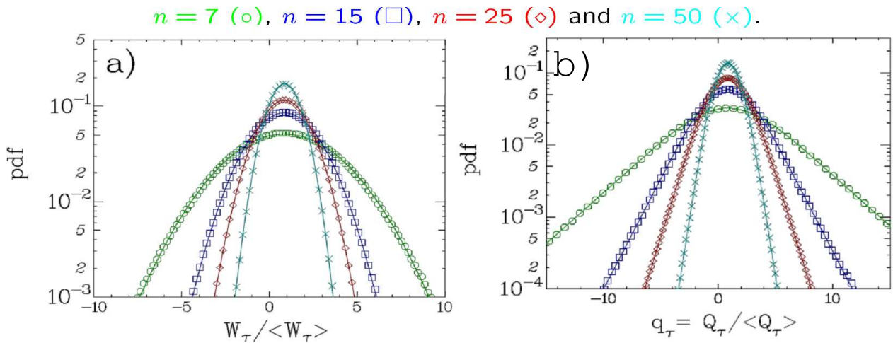
Figure 7: Sinusoidal forcing. a) Pdf of W_\tau b) Pdf of Q_\tau . The continuous lines in this figures are not fits but are analytical predictions obtained from the Lnagevin dynamics as discussed in sect.3.4
