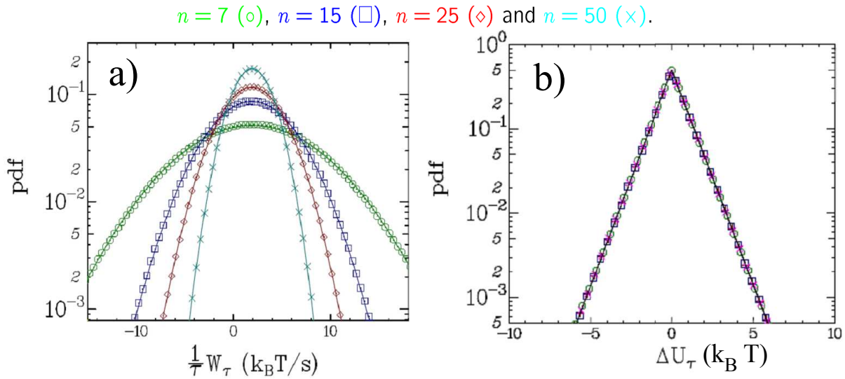
Figure 6: Sinusoidal forcing. a) Pdf of W_\tau b) Pdf of \Delta U_\tau
