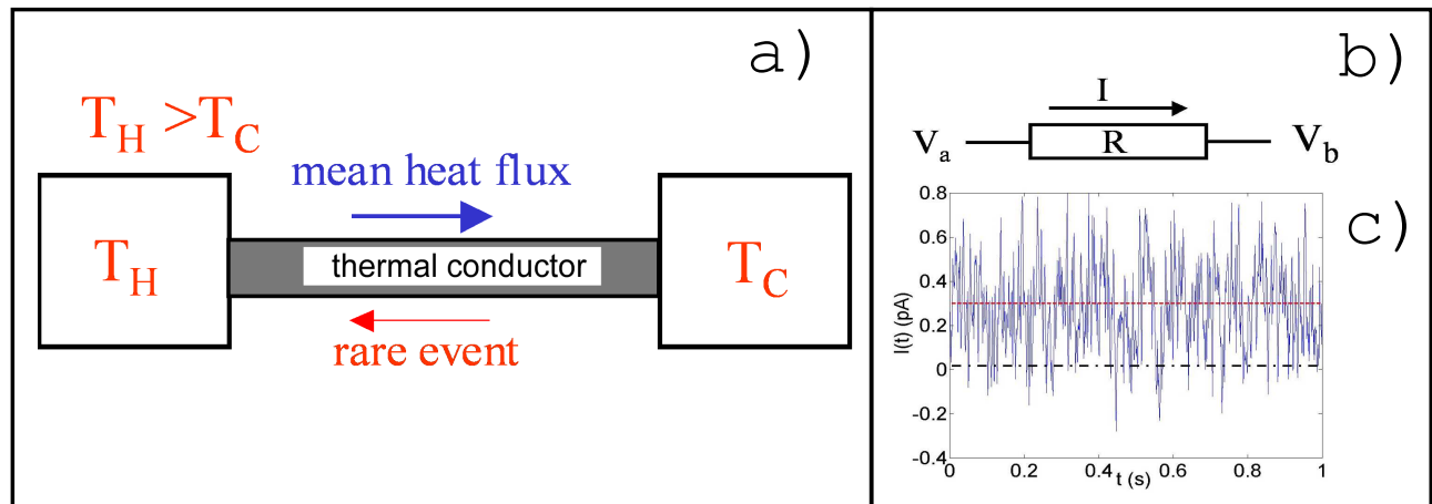
Figure 1: a) Schematic representation of a conductor whose extremities are contact with two heat baths at temperature T_H and T_C with T_H > T_C . b) Electrical analogy. A conductor of electrical resistance R and kept at a temperature T is submitted to a potential difference V = V_a - V_b . c) Instantaneous current I flowing into the resistance using R = 10M\Omega , T = 300K and \tau_0 = 2ms .
