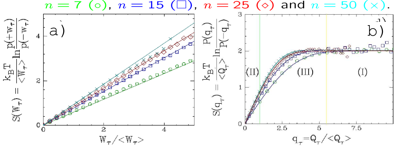
Figure 8: Sinusoidal forcing. Symmetry functions for SSFT. a) Symmetry functions S(w_\tau) plotted as a function of w_\tau for various n . For all n the dependence of S(w_\tau) on w_\tau is linear, with slope \Sigma_w(\tau) . b) Symmetry functions S(q_\tau) plotted as a function of q_\tau for various n . The dependence of S(q_\tau) on q_\tau is linear only for q_\tau < 1 . Continuous lines are theoretical predictions.
