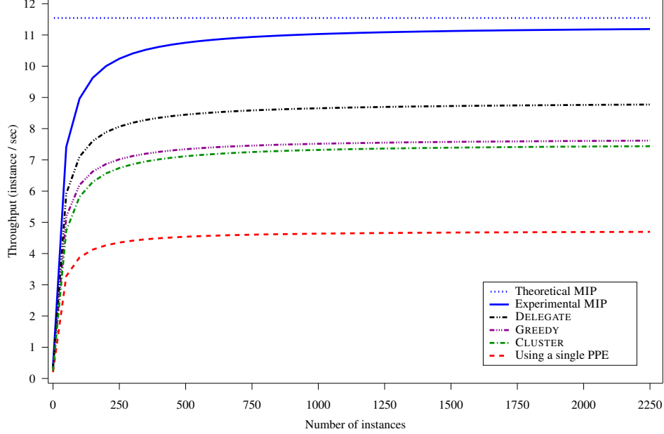
Figure 10: Throughput achieved depending on the number of instances.
