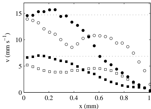
FIG. 10: Individual velocity profiles recorded at T = 39.4^\circ\text{C} for \dot{\gamma} = 7 \text{ s}^{-1} ( \blacksquare, \square ) and \dot{\gamma} = 15 \text{ s}^{-1} ( \bullet, \circ ). The dotted lines indicate the corresponding rotor velocities v_0 .
