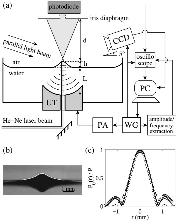
FIG. 1: (a) Experimental setup. (b) Picture of the steady free surface deformation (and of its reflection on the air-water interface) observed for a pressure amplitude P = 0.93 MPa at focus and f = 2.46 MHz. Solid white line: predicted shape using Eq. (1). (c) Symbols: rescaled amplitude of the pressure field of the input beam measured in the focal plane. Solid line: prediction from Ref. [20]. Dashed line: Gaussian approximation.
