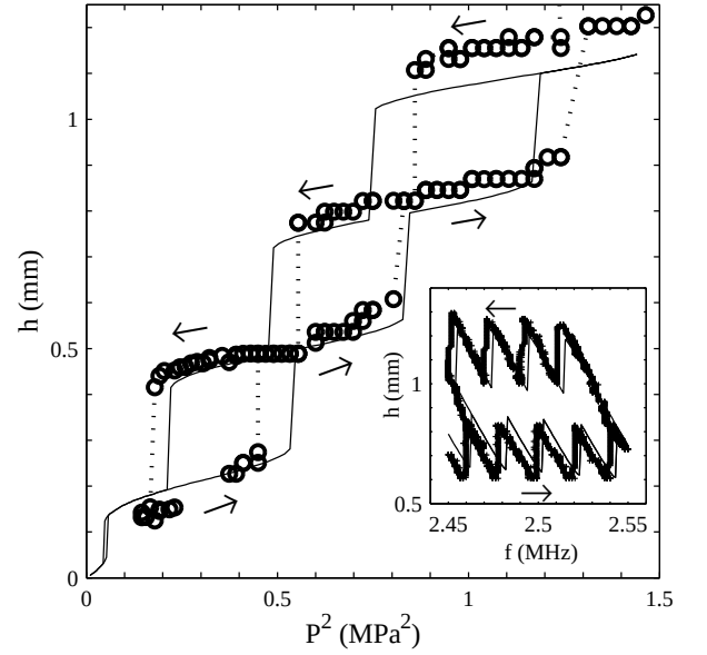
FIG. 2: Surface deformation height h versus the square of the pressure amplitude P at focus due to the input beam ( f = 2.5 MHz). Symbols: experiment. Solid line: theoretical prediction using the model illustrated in Fig. 3. Inset: h versus the acoustic frequency f at P = 0.97 MPa. Symbols: experiment. Solid line: theoretical prediction.
