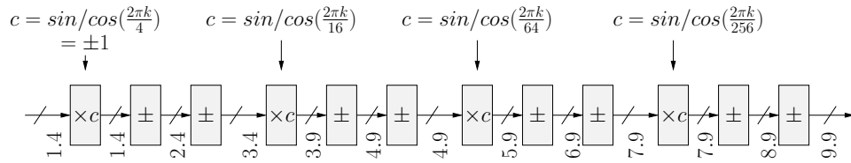
Fig. 3: Fixed-point precisions in the FFT. All the operations shown are complex operations.
