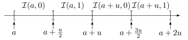
Fig. 2. Binary canonical RN-representations as intervals.
