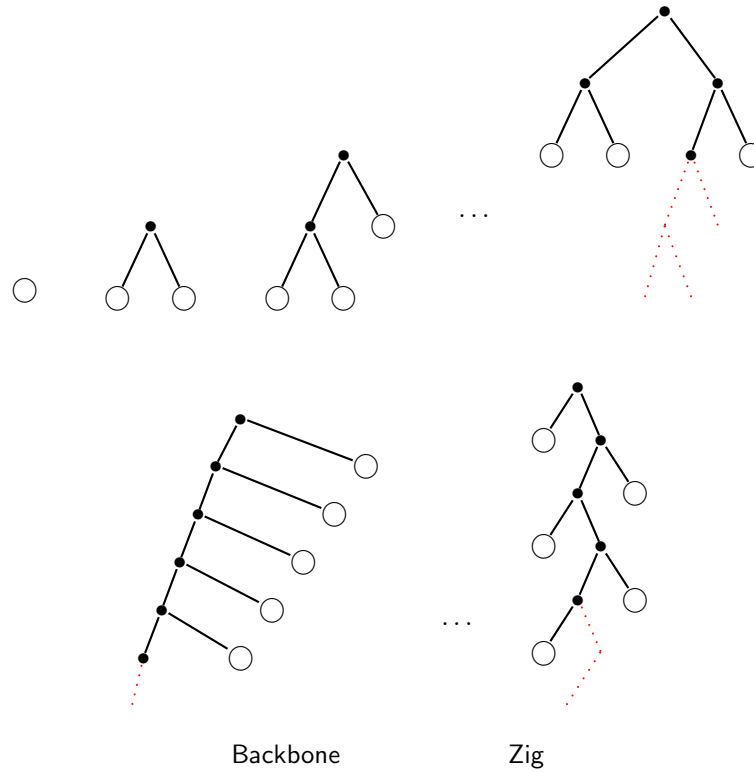
Figure 2.3: Coinductive binary trees
