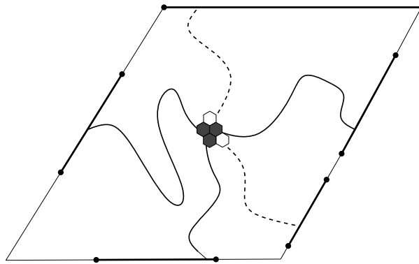
Figure 13: Only one site per rectangle can satisfy the following topological picture.
