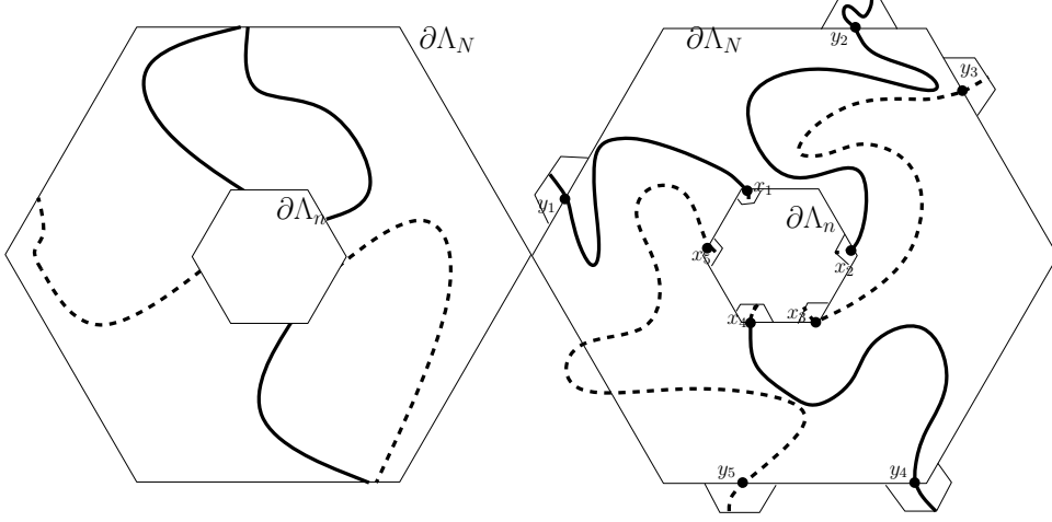
Figure 11: On the left, the five-arm event A_{ocooc}(n, N) . On the right, the event A_{ocooc}^{sep}(n, N) with well-separated arms. Note that these arms are not at macroscopic distance of each others inside the domain, but only at their end-points.
