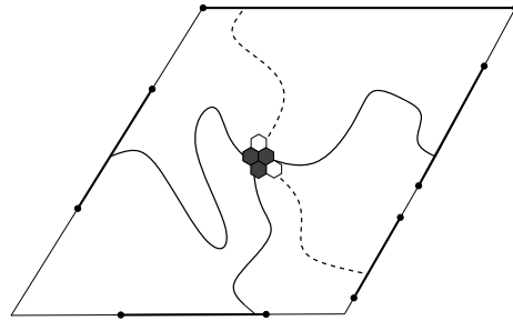
FIG 9. The landing sequences used to prove an upper bound on the probability of the 5-arm event. At most one site with five such arms exists.
