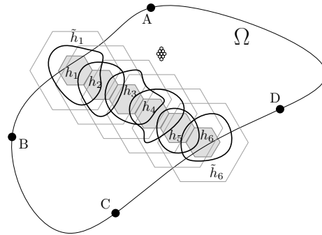
FIG 4. Circuits in annuli linking two arcs of a topological rectangle. If each of these annuli contains an open circuit disconnecting the interior from the exterior boundary, we obtain an open path connecting the two sides.
