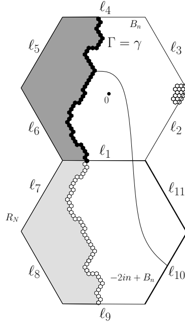
FIG 2. The dark gray area is the set of sites which are discovered after conditioning on \{\Gamma = \gamma\} . The white area is \Omega_\gamma .
