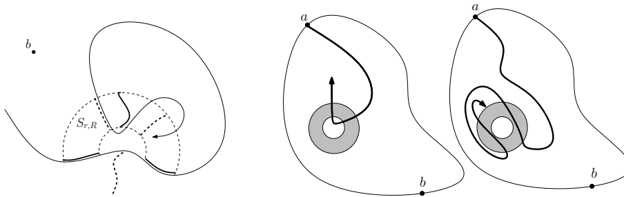
FIG 7. Left: An example of a fjord. Seen from b , the h -capacity (roughly speaking, the size) of the hull does not grow much while the curve is in the fjord. The event involves six alternating open (in plain lines) and closed (in dotted lines) crossings of the annulus. Right: Conditionally on the beginning of the curve, the crossing of the annulus is unforced on the left, while it is forced on the right.
