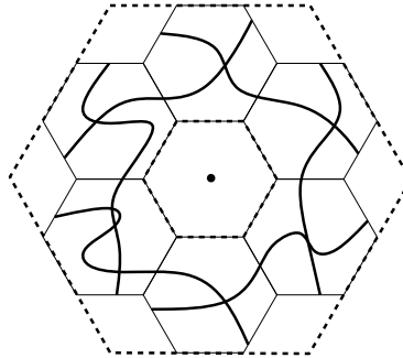
FIG 3. Six “rectangles” which, when crossed, ensure the existence of a circuit in the annulus.
