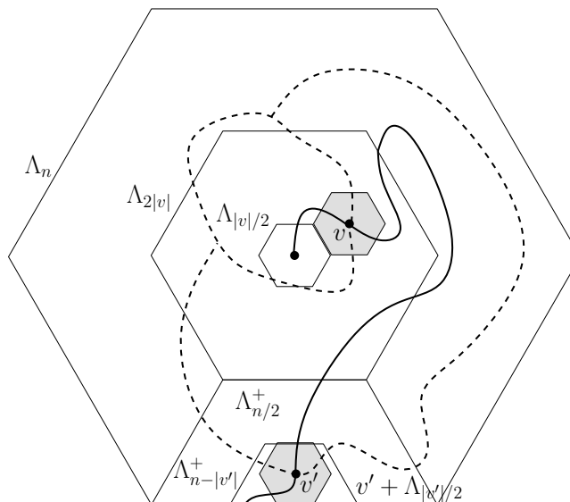
FIG 10. The event that v and v' are pivotal for A_1(n) . The dotted line corresponds to a closed circuit.
