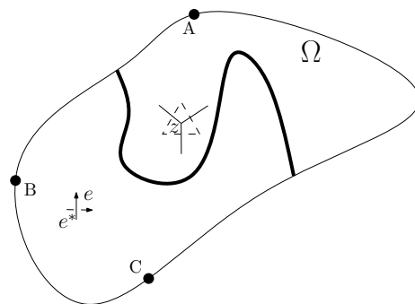
FIG 5. Picture of the event E_{A,\delta}(z) . Also depicted is one oriented edge e with its associated dual edge e^* . The graph \mathbb{T}_\delta is drawn with dotted lines while its dual \mathbb{H}_\delta is drawn with solid lines.
