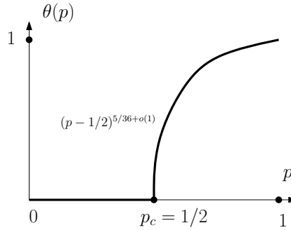
FIG 1. Cluster density with respect to p . Non-trivial facts in this picture include p_c = 1/2 , \theta(p_c) = 0 and the behavior of p \rightarrow \theta(p) near the critical point.
