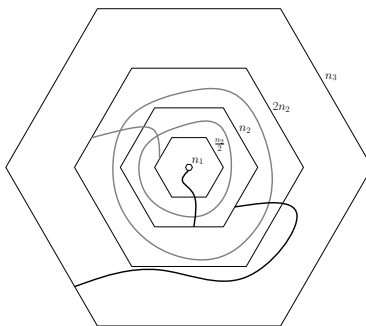
FIG 8. The paths in the annuli \Lambda_{n_3} \setminus \Lambda_{n_2} and \Lambda_{n_2} \setminus \Lambda_{n_1} are in black. A combination of two circuits connected by a path (in gray) connects the paths together. The combination of gray paths in the middle occurs with probability bounded away from 0 thanks to crossing estimates (Theorem 2.1 and Corollary 2.3).
