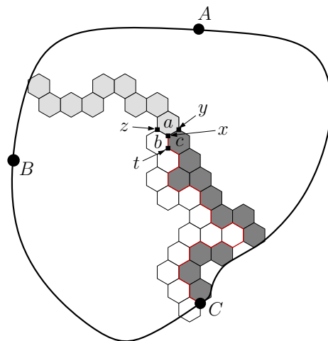
FIG 6. The dark gray and the white hexagons are the hexagons on \bar{\Gamma} , \Gamma being in black.
