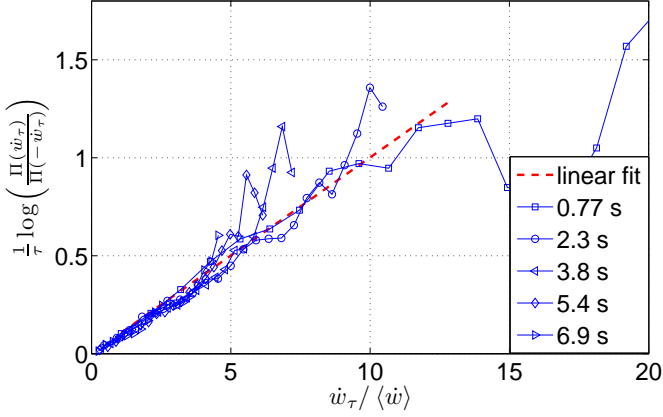
Fig. 6: The asymmetry function \frac{1}{\tau} \log \left( \frac{\Pi(\dot{w}_\tau)}{\Pi(-\dot{w}_\tau)} \right) is plotted against \dot{w}_\tau / \langle \dot{w} \rangle , for the same 5 time-lags as on previous figure ( \square : 0.77 s, \circ : 2.3 s, \triangleleft : 3.8 s, \diamond : 5.4 s, \triangleright : 6.9 s, i.e. 980 to 8.9 10^3 \tau_c , where \tau_c \simeq 7.8 \cdot 10^{-4} s). A linear fitting is performed, shown only at the smallest \tau (dashed line).
