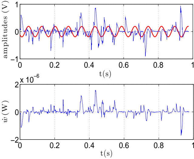
Fig. 3: Top: time-series of the imposed sine current ( I \simeq 200\text{ }\mu\text{A} ), and the induced voltage. For homogeneity and comparison, both have been plotted in Volts: R I(t) (bold), and for readability, e has been enlarged by a factor 100 (thin). Bottom: in the same time-scale, the corresponding energy flux \dot{w}(t) is plotted. The mean power given is \langle \dot{w} \rangle \simeq 7.3\text{ nW} . The acceleration is a \simeq 56\text{ ms}^{-2} .
