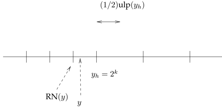
Figure 3: When y_h is a power of 2, |y_h - y| < \frac{1}{2}\text{ulp}(y_h) does not necessarily imply that y_h = \text{RN}(y) .
