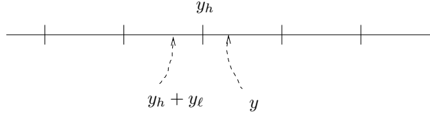
Figure 2: Illustration of Property 1: when (y - y_h) and y_\ell have different signs, y is closer to y_h than to y_h + y_\ell , which implies y_h = \text{RN}(y) .
