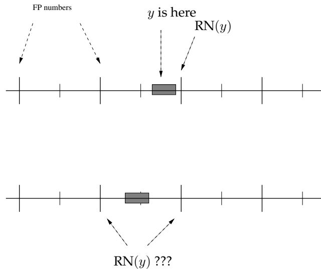
Figure 1: Given an approximation y_1 to y = f(x) and a bound \epsilon_1 on the approximation error, we know that y lies in an interval I_1 . In the first case, all elements of I_1 round to the same floating-point number, so that we can return \text{RN}(y) . In the second case, a new, more accurate, approximation y_2 must be computed.
