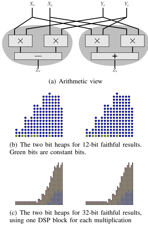
Fig. 4. Complex multiplication as two bit heaps
