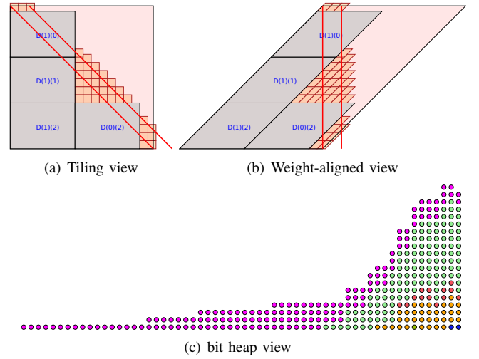
Fig. 2. 53 \times 53 -bit multiplier faithful to 53-bit, for Virtex5. The bits between the two red lines are guard bits needed for a faithful result. Different colors in the bit heap indicate bits arriving at different instants.
