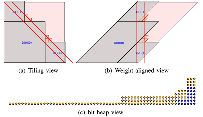
Fig. 3. 53 \times 53 -bit faithful multiplier for Stratix IV.
