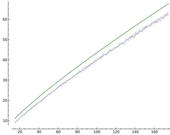
Figure 6: Average depth of variables and curve \frac{2n}{\ln(n)}
